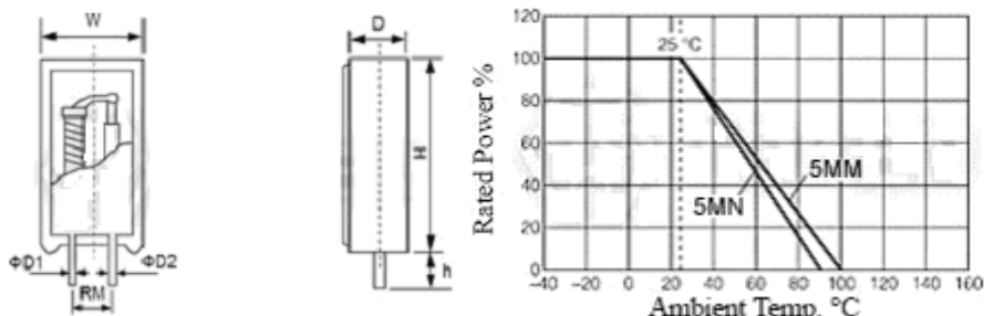
Power Derating Curve
